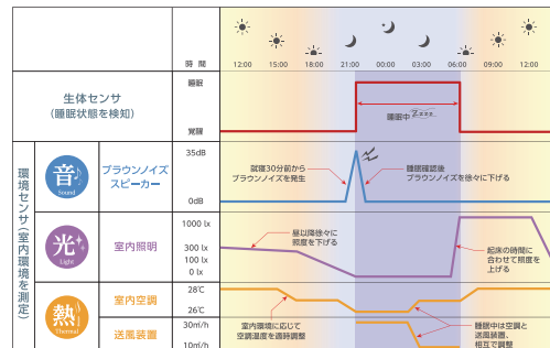
病室内の環境や患者の睡眠状態に合わせた設備の制御イメージ Image of Equipment Control According to the Environment in the Hospital Room and the Sleep State of the Patient
